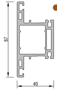
MULLION PROFILE R 21601-02003 : ROBLE
