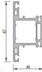
MULLION PROFILE 21601 - 02000 : WHITE
