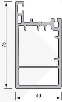
SASH PROFILE 21601 - 01000 : WHITE
