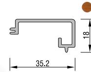
SASH COVER PROFILE R 21601-05003 : ROBLE
